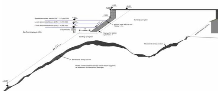
1 Snitt utfylling 1 1 : 200
