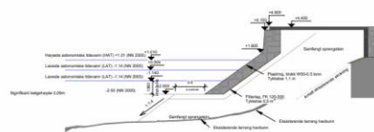
3 Snitt utfylling 3 1 : 200
