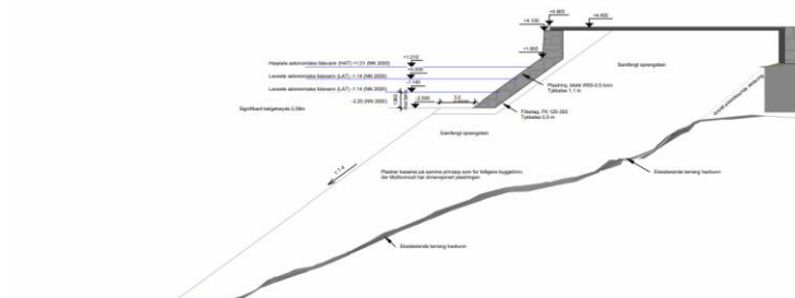
1 Snitt utfylling 1 1 : 200
